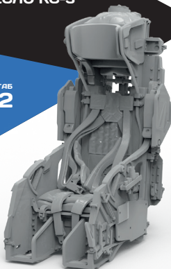
Ejection seat KS-3 (suitable for Su-7, Su-15, Su-17 all model kits)
